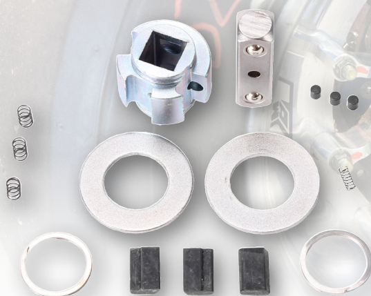
13212 Repair Kit
